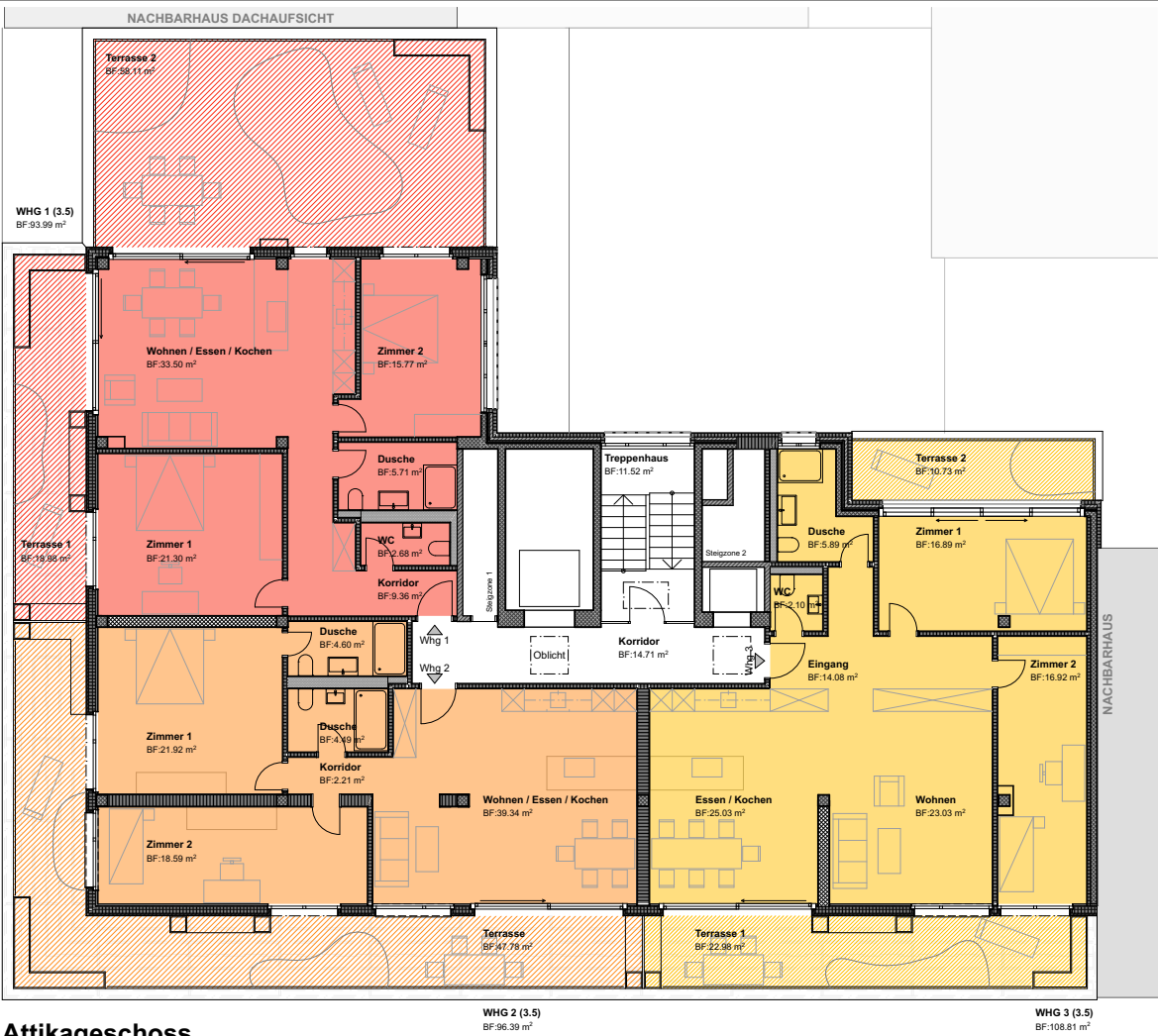
Attikageschoss
