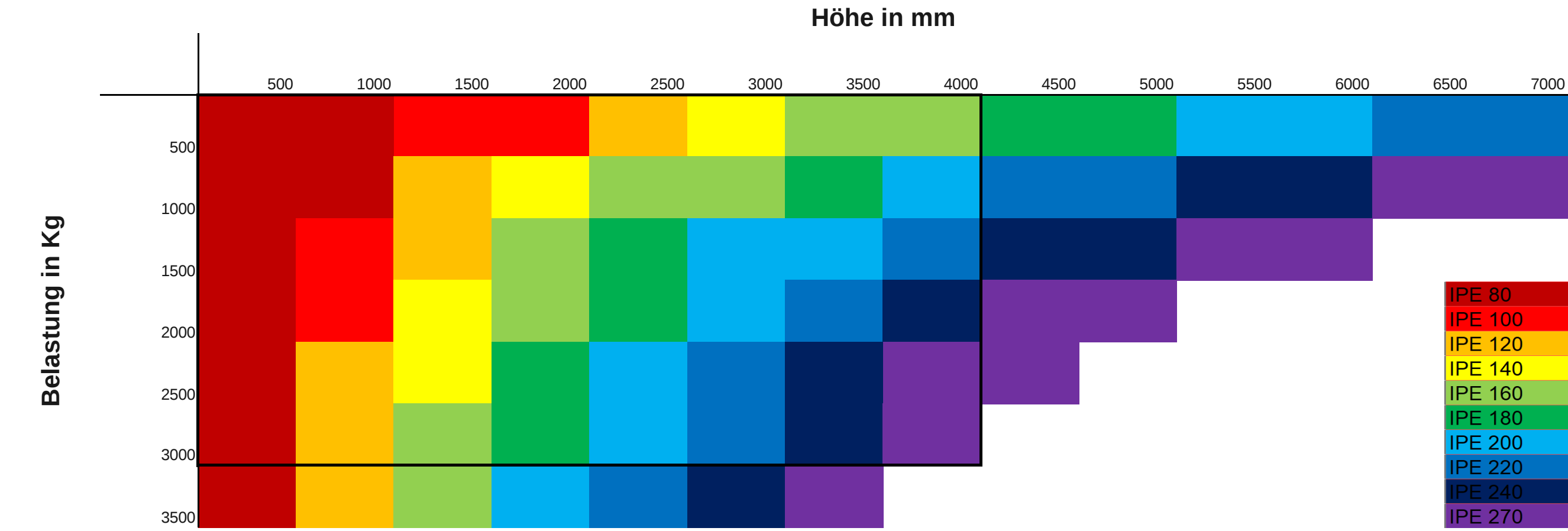
IPE Profile
