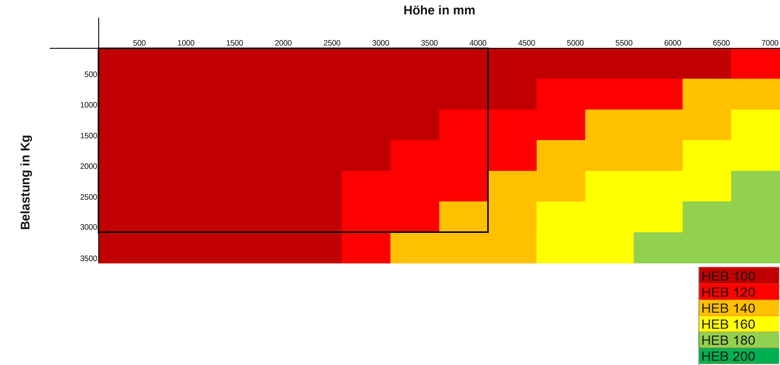
HEP Profile
