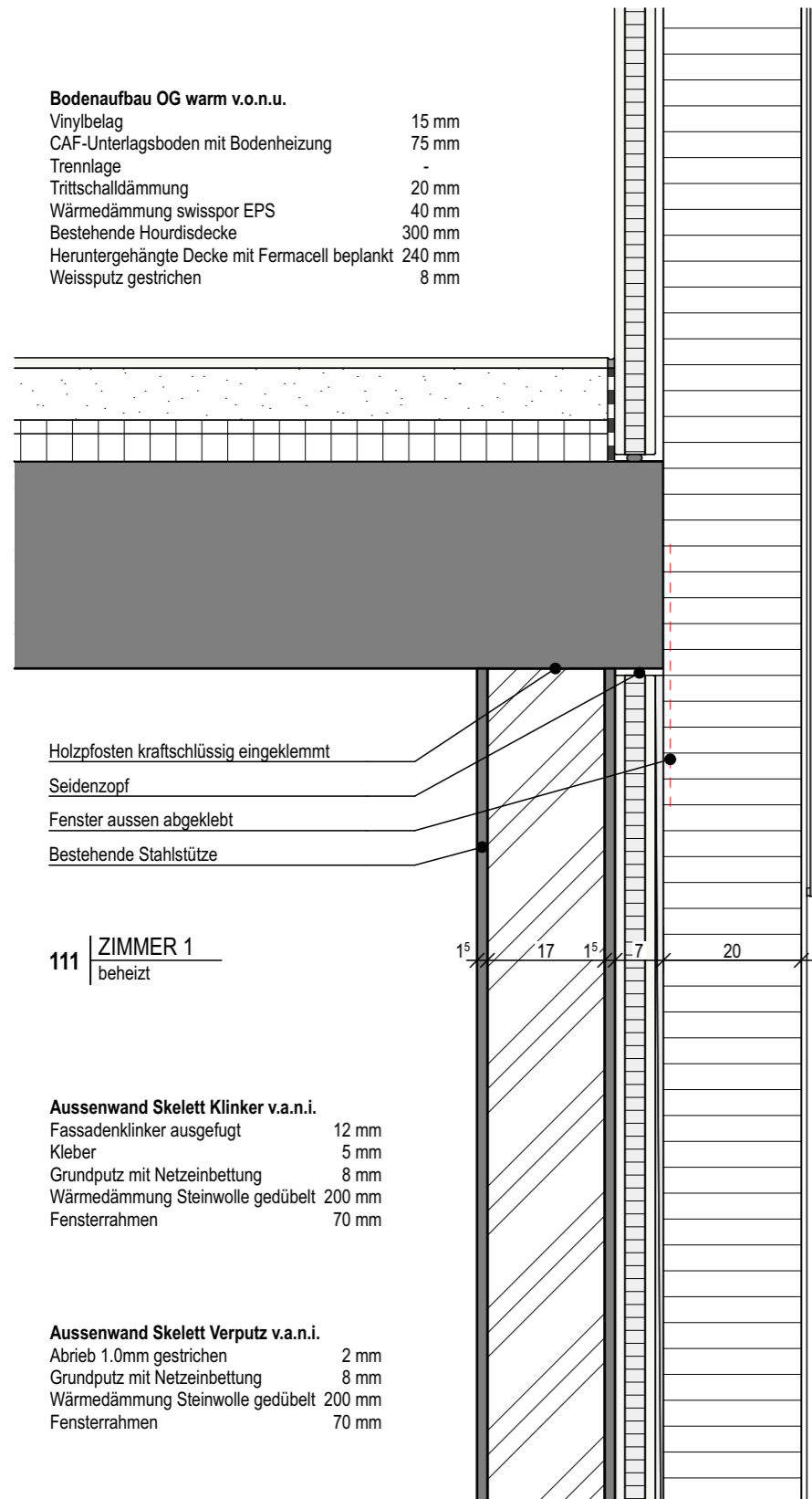
DETAIL STATIK 1:10
